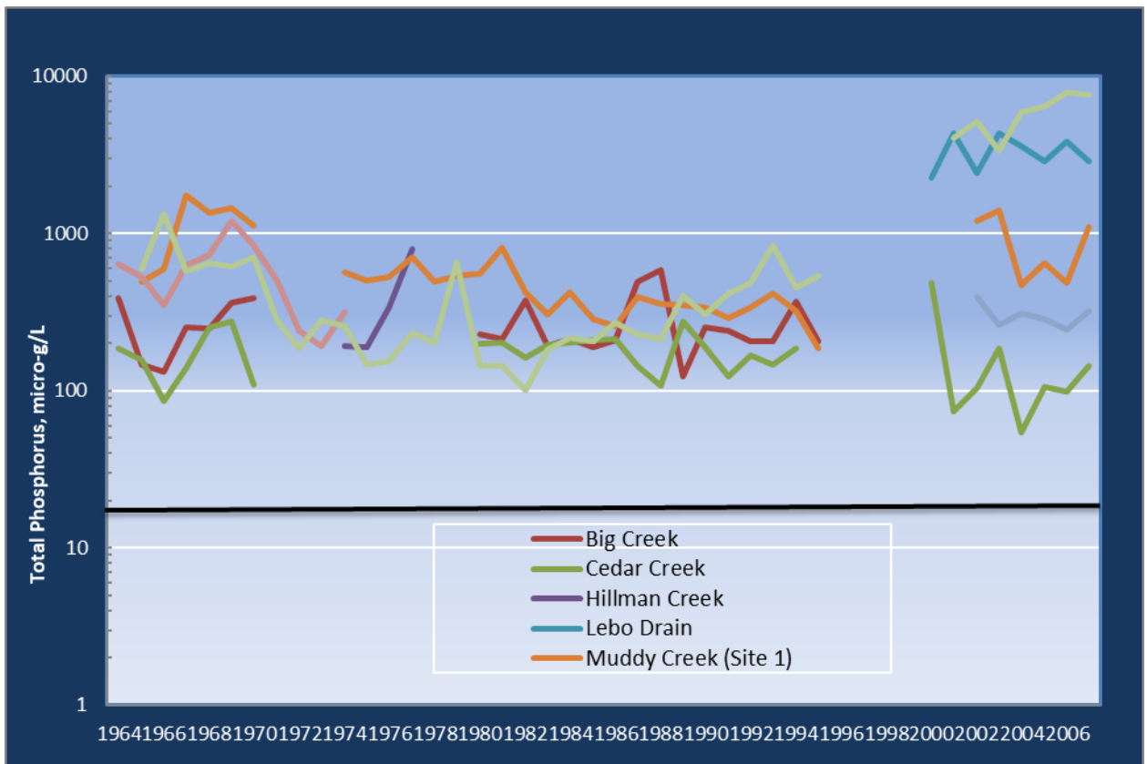
Figure 2.3: Long-term annual mean total phosphorus concentration trends in the streams of the Essex Region Watershed that drain into Lake Erie.
