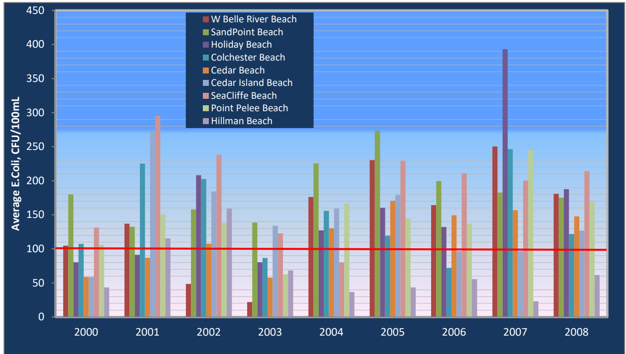
Figure 2.8: Annual mean E. coli levels observed at 9 of the public beaches in the Essex Region during summer seasons of 2000 to 2008
